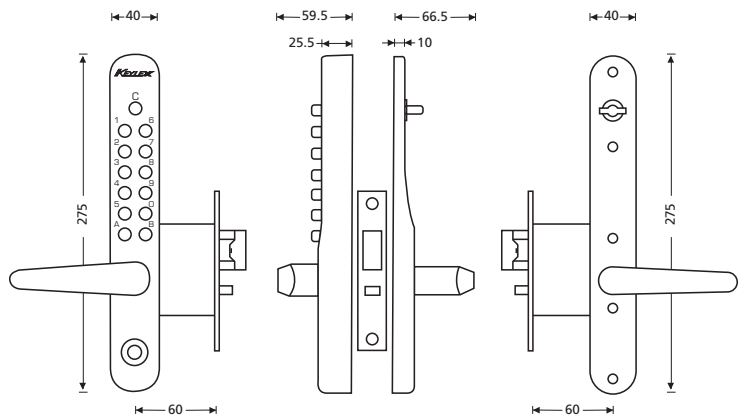
REL.K800 Model with Mortice Double Throw Deadlocking Latch
